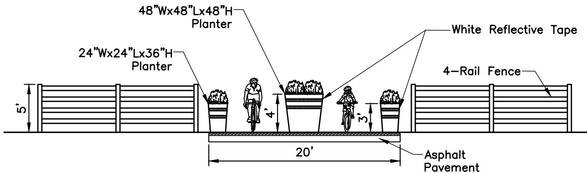
Elevation View
