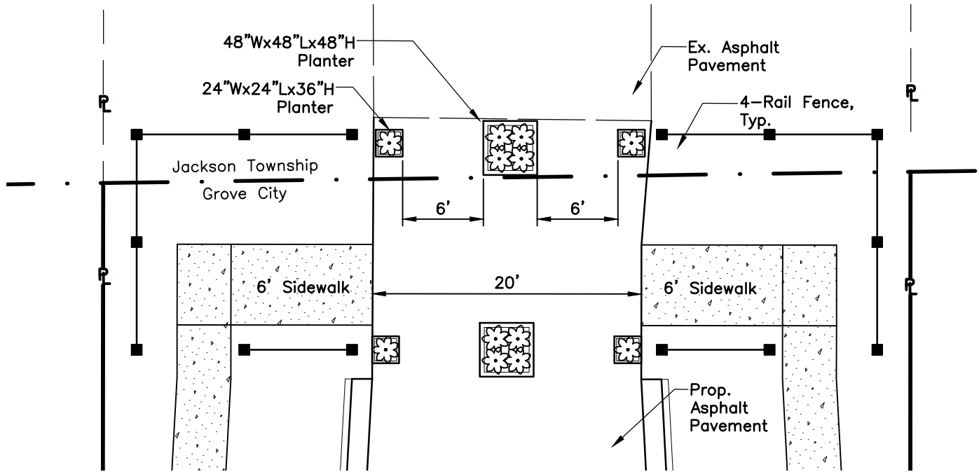
Plan View
